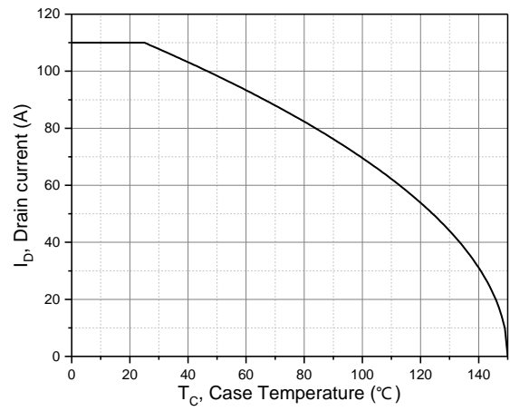
Figure 8. Drain current
