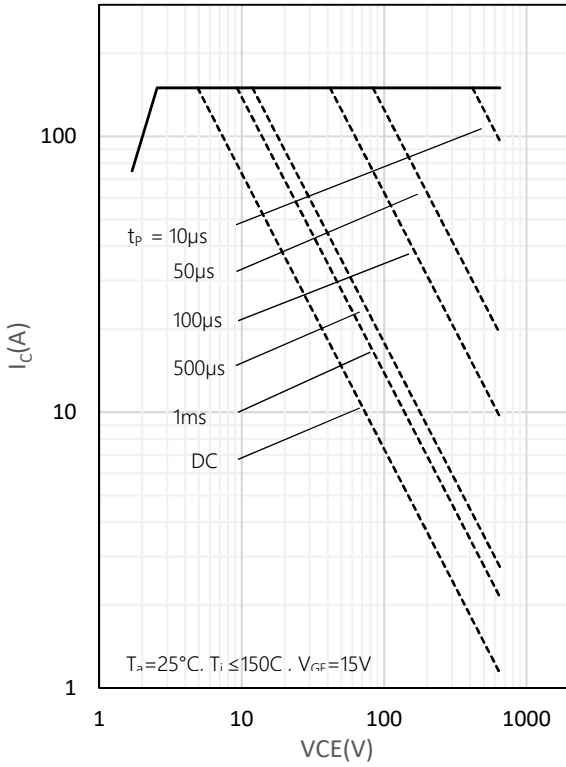
Fig. 1 FBSOA characteristics
