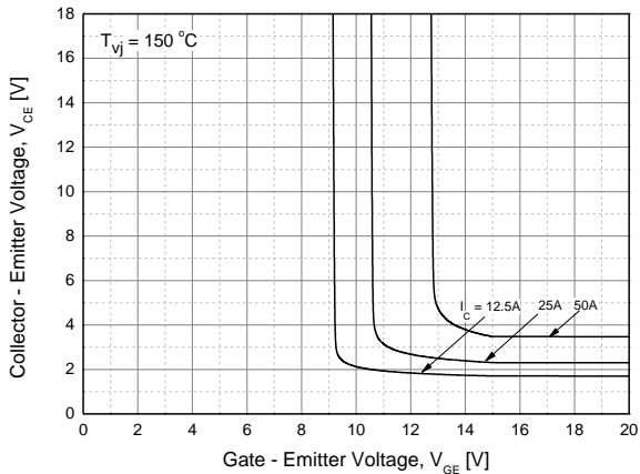
Fig. 5 IGBT Saturation Voltage vs. Gate Bias
